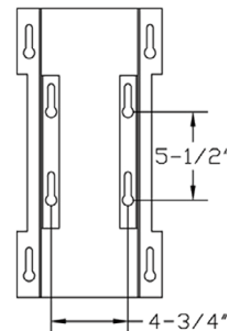
BRACKET MOUNT
